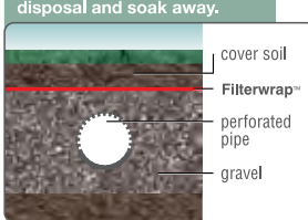
8. Underground waste disposal and soak away.
