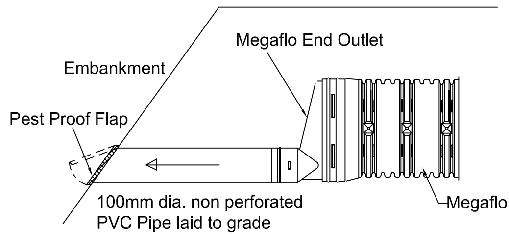
Typical End Outlet 1 (Outlet to Natural Surface)
