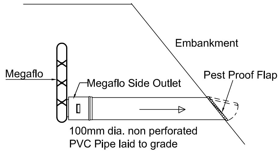
Typical Side Outlet 1 (Outlet To Natural Surface)
