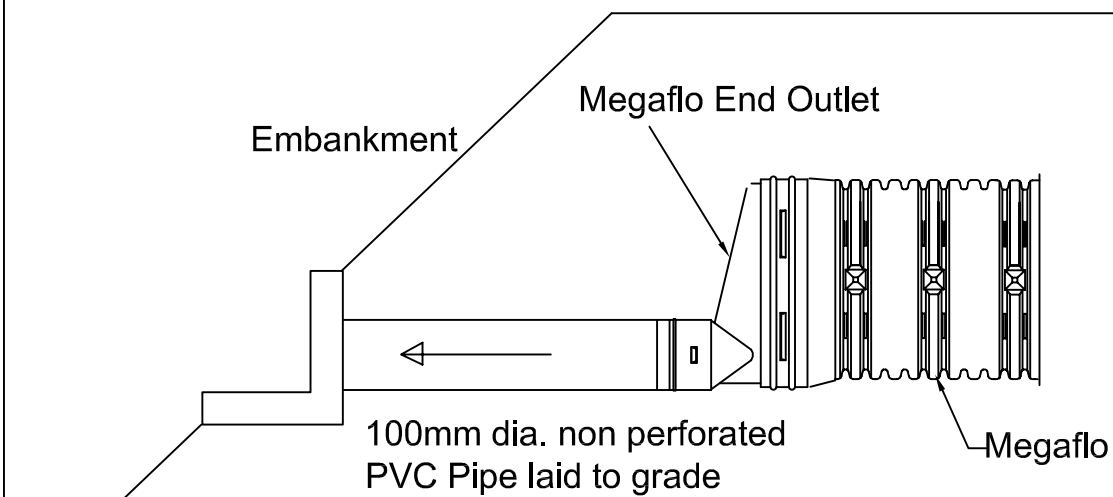
Typical End Outlet 2 (Precast Headwall)
