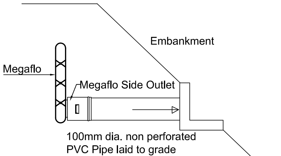
Typical Side Outlet 2 (Precast Headwall)
